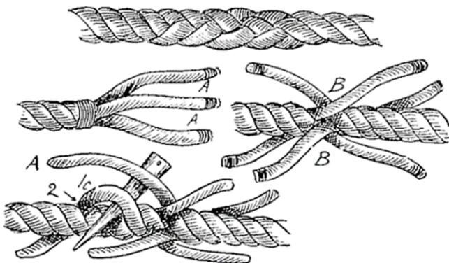
FIG. 106.—Short splice.
